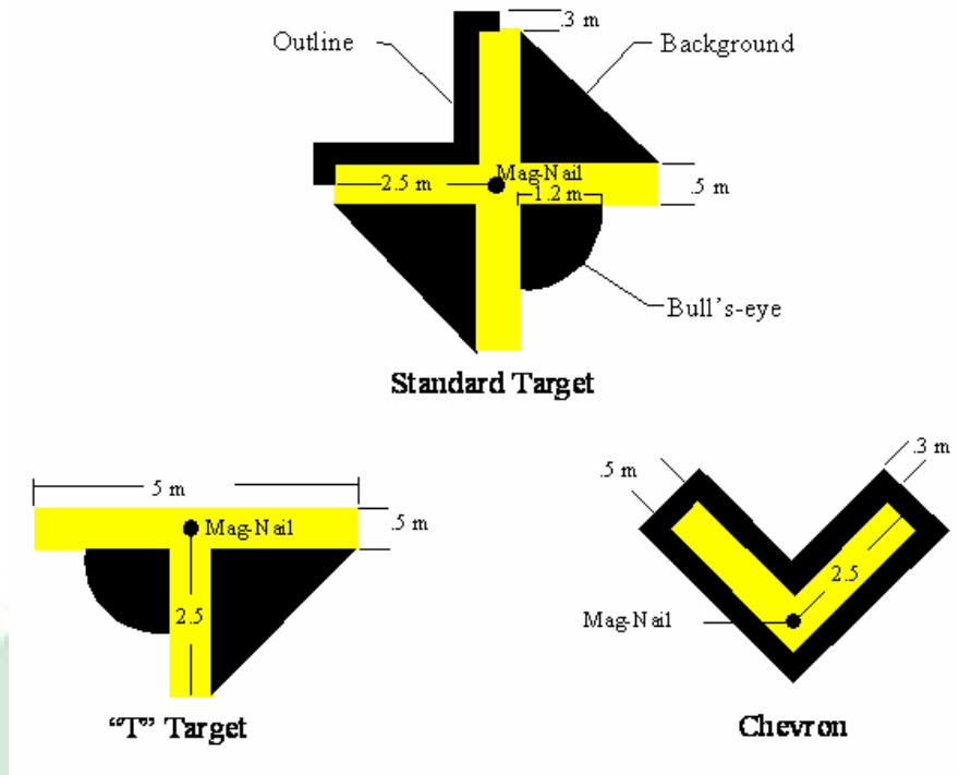
Figure 1. Standard Photogrammetry Targets. Modified from the Survey Engineering Department at Ferris State University.
