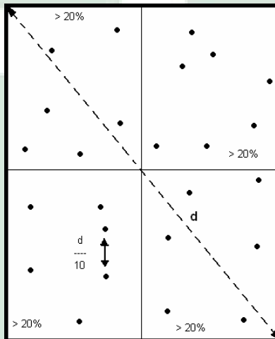
Figure 4. Hypothetical Distribution of Sample Points. Modified from Congalton and Green, 2009.
